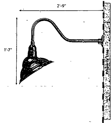
Gooseneck Lamp Side View
