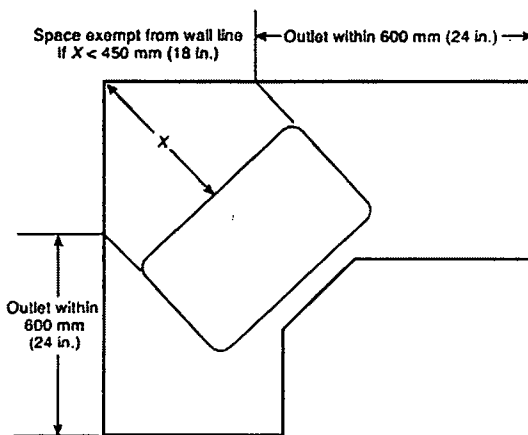
Range, counter-mounted cooking unit mounted in corner
