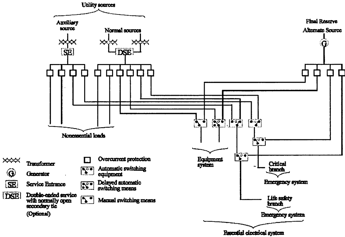
Insert Figure 517.29(B)(4)(b):
