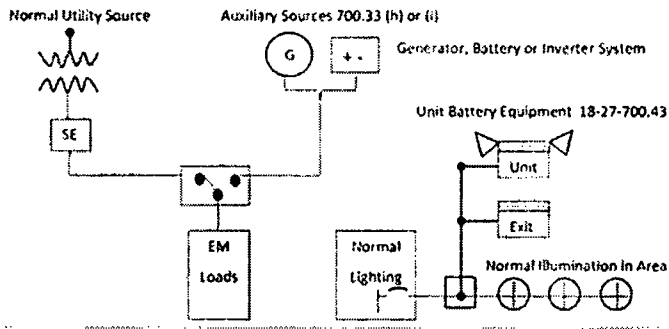
Figure 700.21-22 Typical of Either System II or System III Emergency Systems.
