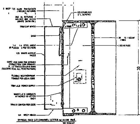
SCALE 3/32" = 1'
