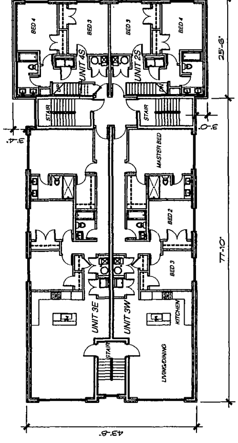
FOURTH FLOOR
