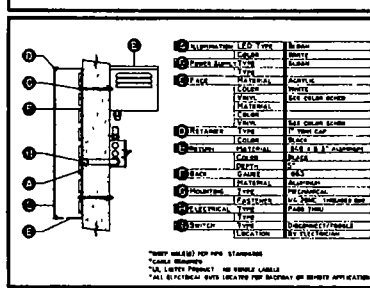
"LOGO & ACCEPTANCE" LED Face Lit Letter Flush Mounted (Returns)
