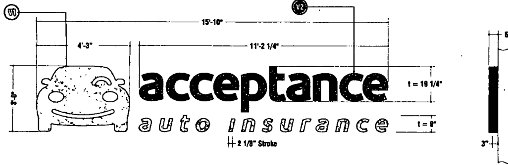
"LOGO & ACCEPTANCE" LED Face Lit Letter Flush Mounted (Returns)
