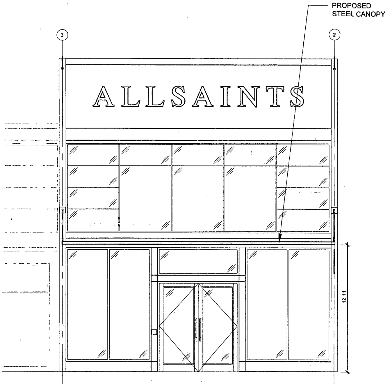
1 ELEVATION CANOPY ENTRANCE SD-1 SCALE 3/16" = 1'-0"
