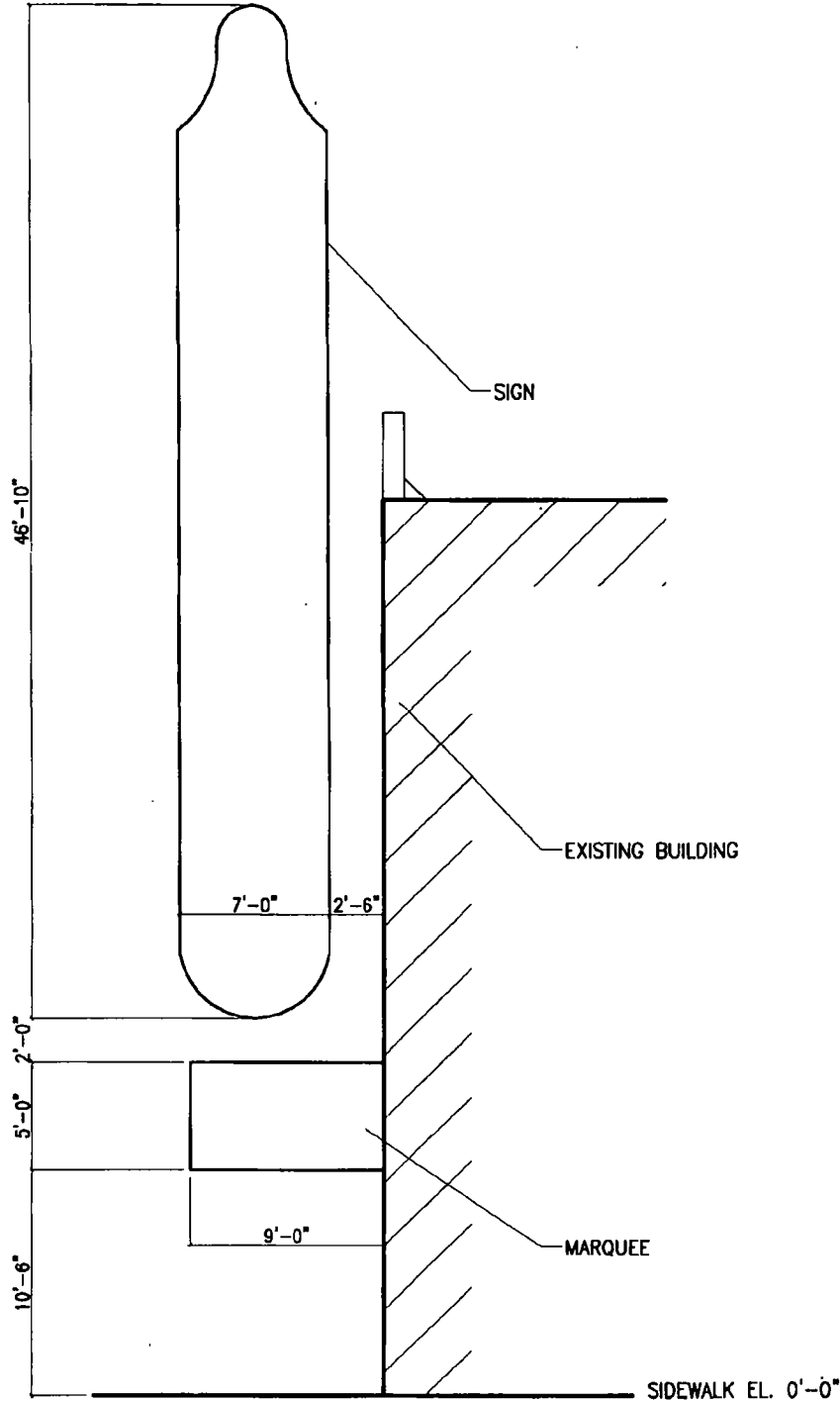
1 MARQUEE AND SIGN SIDE ELEVATION A3.0 Scale: 1/8"=1'0"
