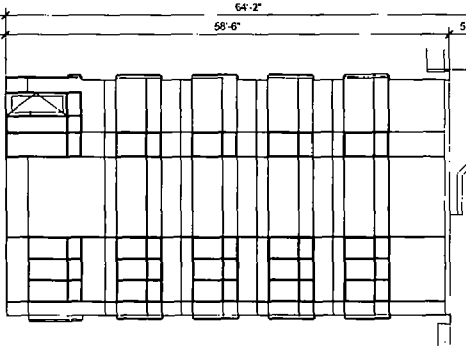
NORTH ELEVATION @ COURTYARD METAL PANEL FACADE AREA 1,497 SF GLASS FACADE AREA 490 SF
