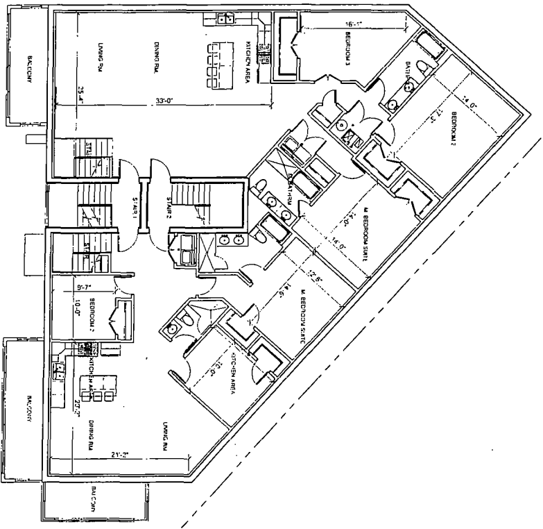
Third Floor Plan Scale: 1/8" = 1'-0"
