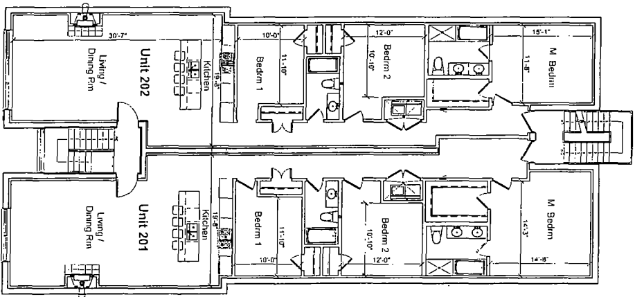
Second Floor Plan Scale 1/8" = 1'-0"
