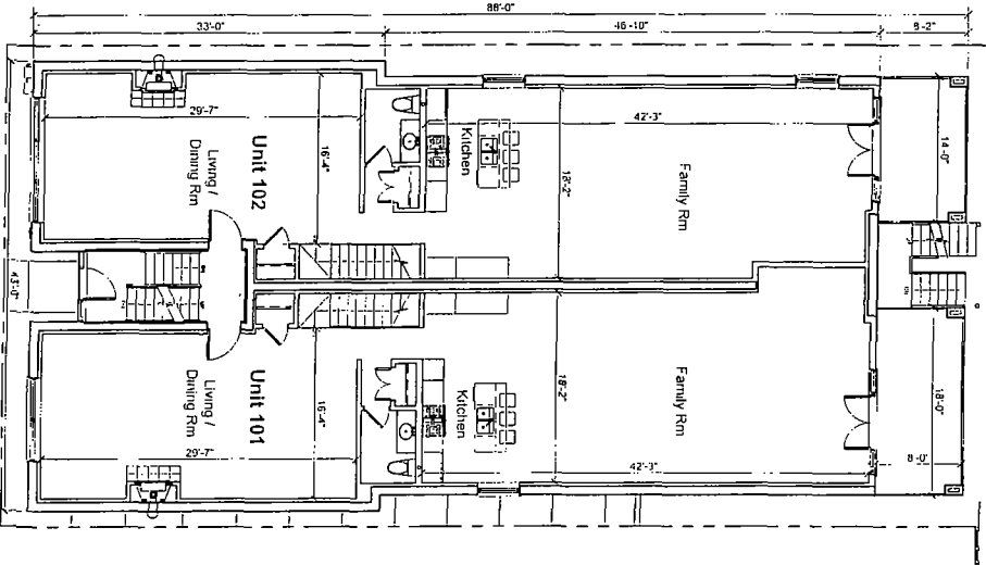
First Floor Plan Scale: 1/8" = 1'-0"
