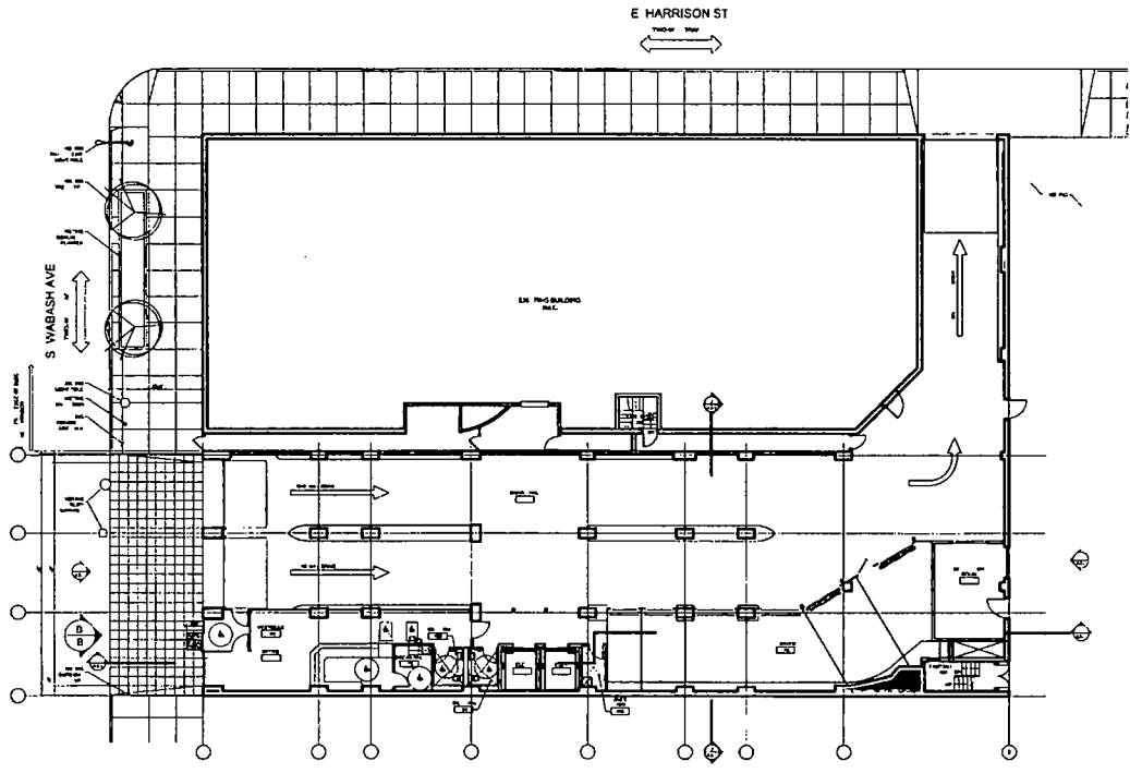
SITE PLAN
