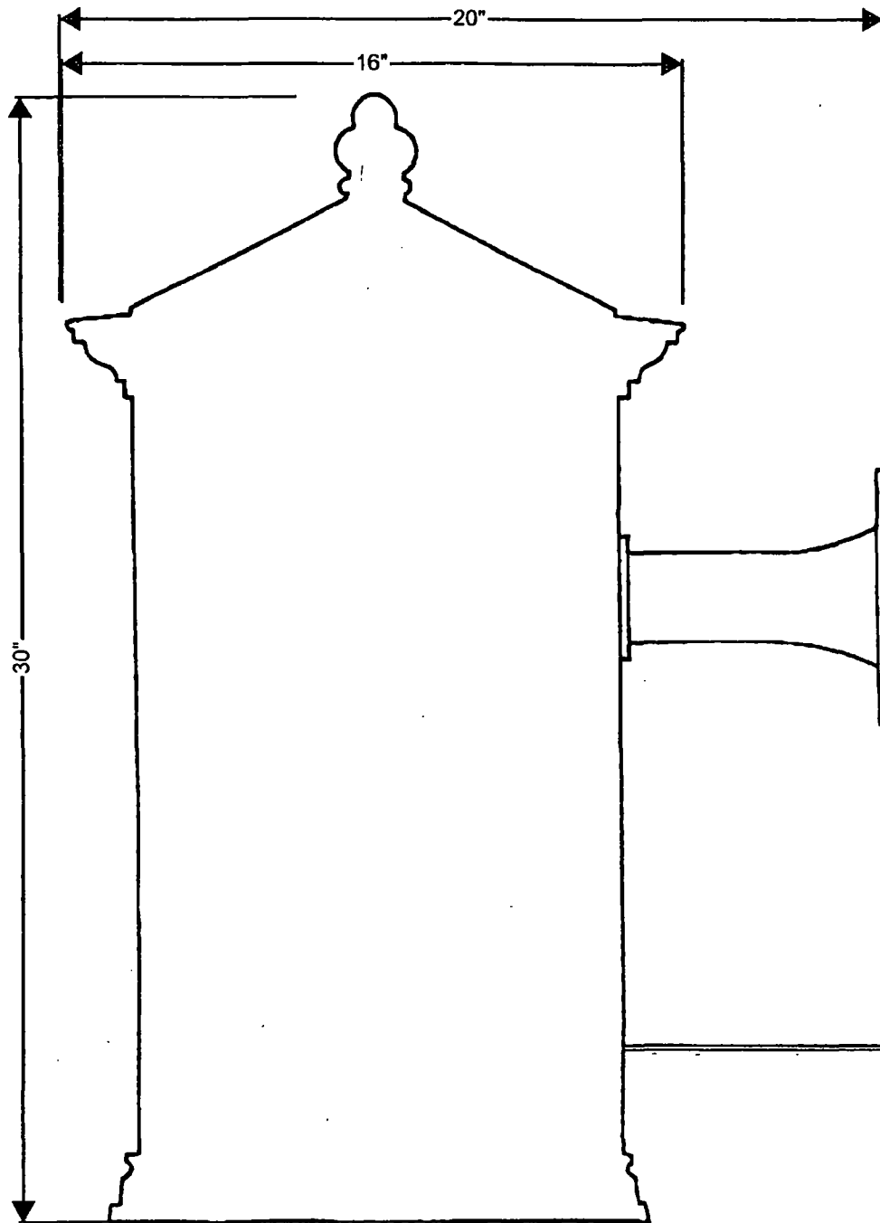
● ● Schematic of Ornamental Light Fixture
