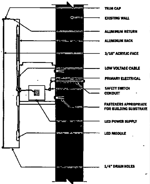
Standard Face Lit - LED Illuminated w/ Raceway
