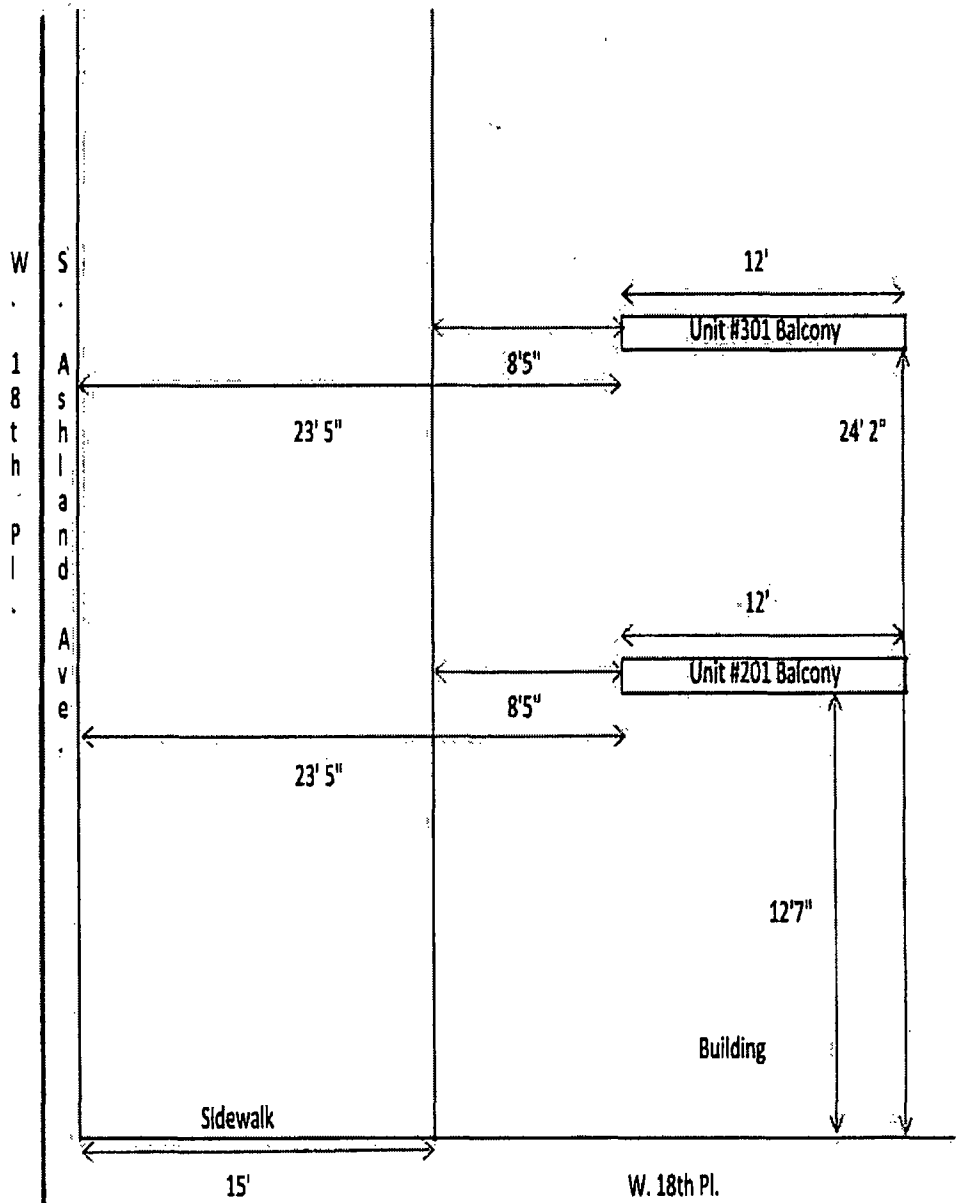
Left sketch: Birds-eye view of NE corner of building (at intersection of S. Ashland Ave. & W. 18th Pl.), showing Unit #301 balcony, which is directly above Unit #201 balcony.
