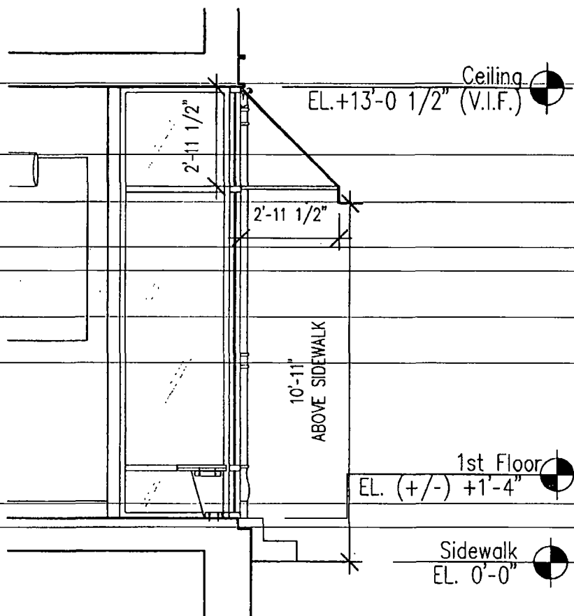
1 PARTIAL SECTION AT STOREFRONT A-7 1/4" = 1'-0"
