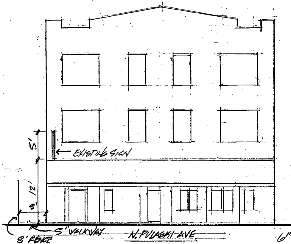
WEST ELEVATION (FRONT FACADE)
