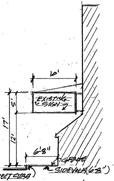
SECTION LOOKING NORTH
