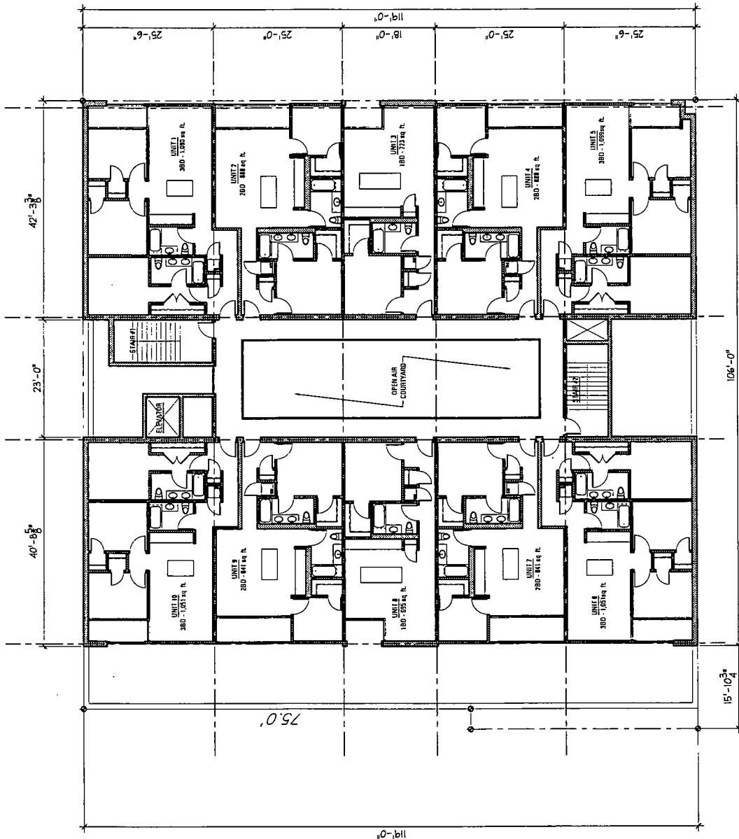
SECOND FLOOR PLAN - 10,394 sq. ft.
