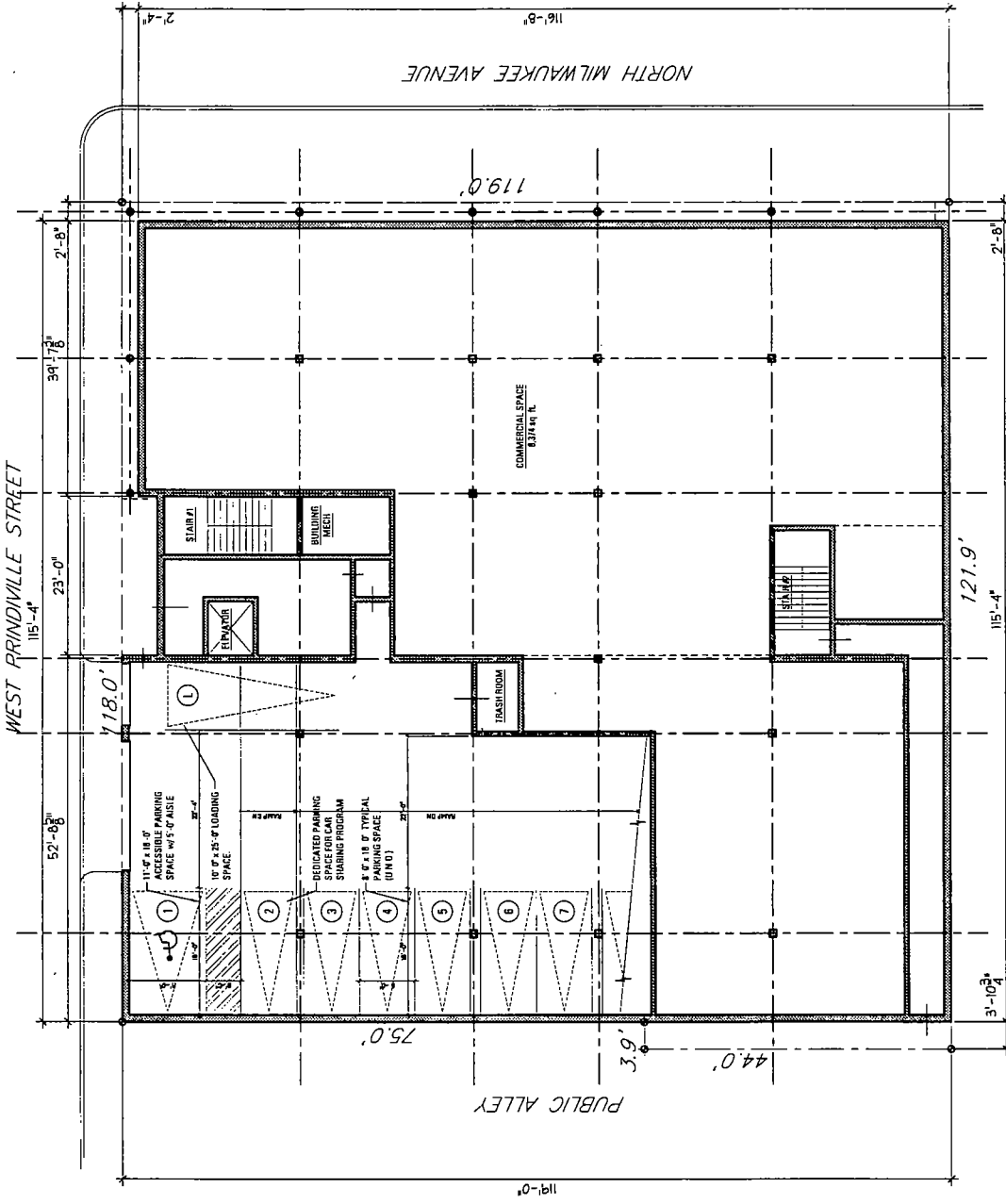
FIRST FLOOR PLAN - 9,739 Sq. ft.
