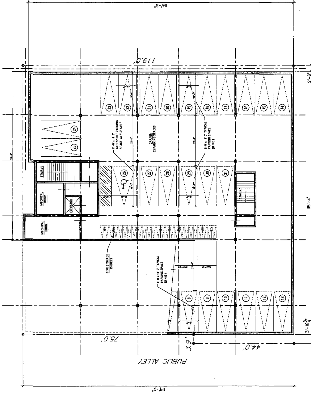
BASEMENT PLAN - 10,693 sq. ft.
