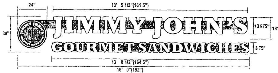
A Front-Lit, Plex-Face Channel Letters, Raceway Mounted • Front View SCALE 3/8" = 1'-0" For Production / For Presentation
