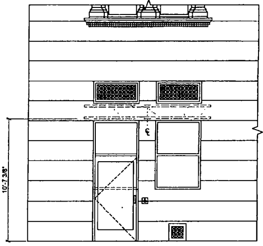
E ELEVATION Scale 1/4"=1'-0"
