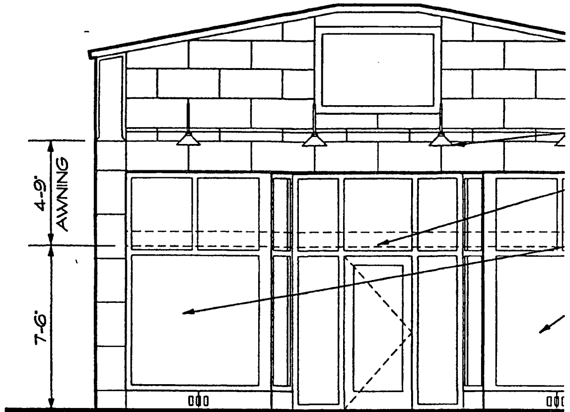
02 Front Elevation Scale 1/4" = 1'-0"
