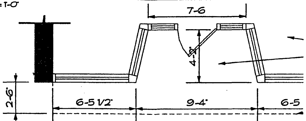
01 Front Entry Construction Plan Scale 1/4" = 1'-0"
