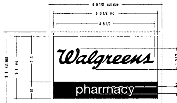
Face Layout/Dimensions 3/4 - 1-0 Cabinet size not provided 2 1/2 retainers
