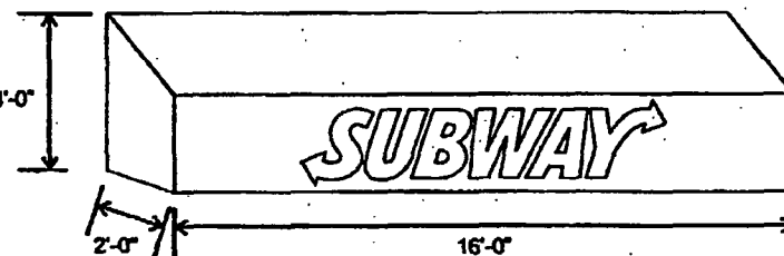
Non-illuminated awning
