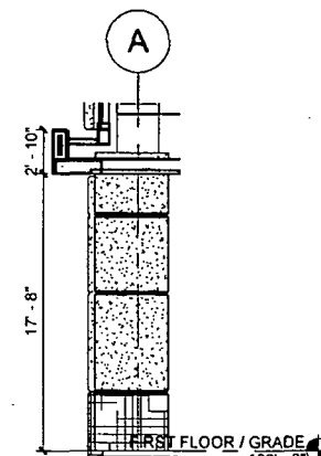
SECTION A OF CANOPY
