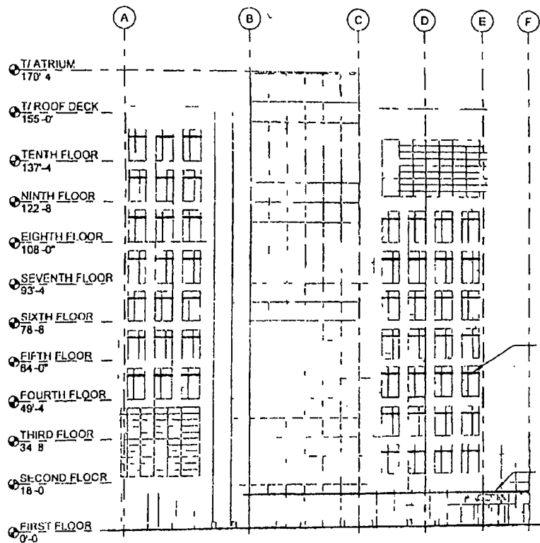
1 SOUTH ELEVATION ENCROACHMENT 1/32" = 1'-0"
