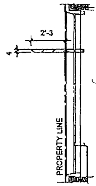
3 SOUTH WINDOW SHADE SECTION 1/4" = 1'-0"
