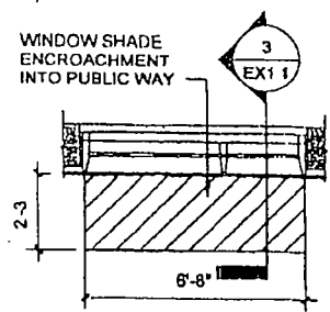
2 SOUTH WINDOW SHADE PLAN 1/4" = 1'-0"
