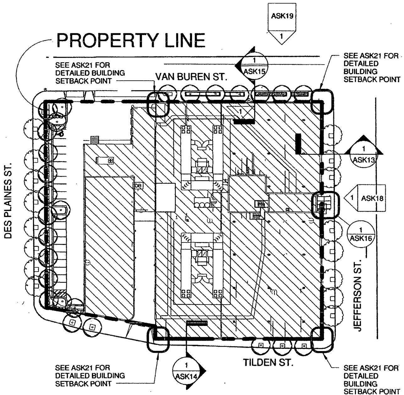
1 ARCHITECTURAL SITE PLAN - PROPERTY LINE 1/64" = 1'-0"
