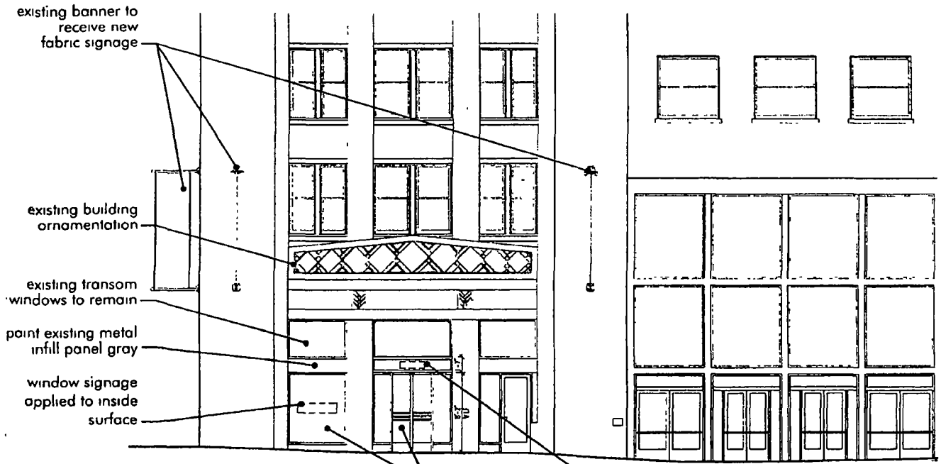
Entry Detail Elevation NTS
