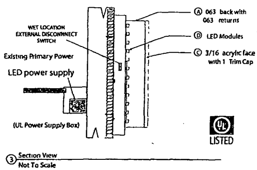
Typical Wireway Mount channel Letters with LED's
