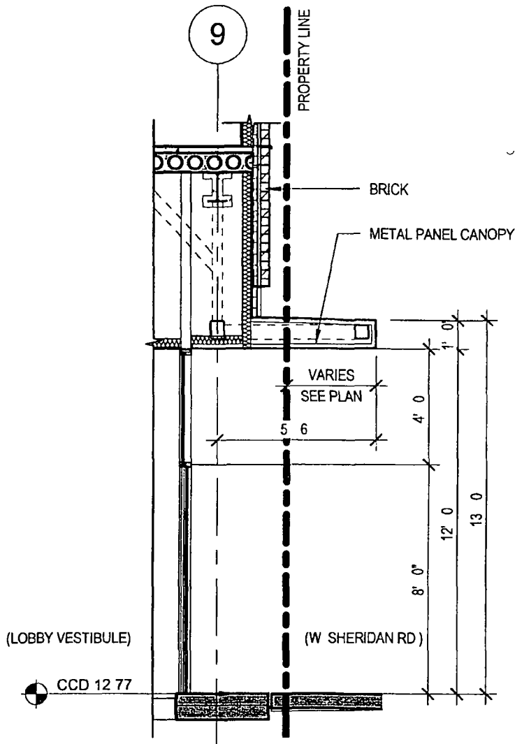
② ENTRANCE CANOPY 1/4" = 1'-0"
