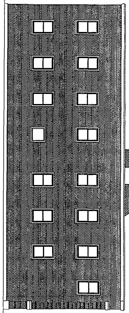
NORTH ELEVATION SCALE: 3/32" = 1'-0"
