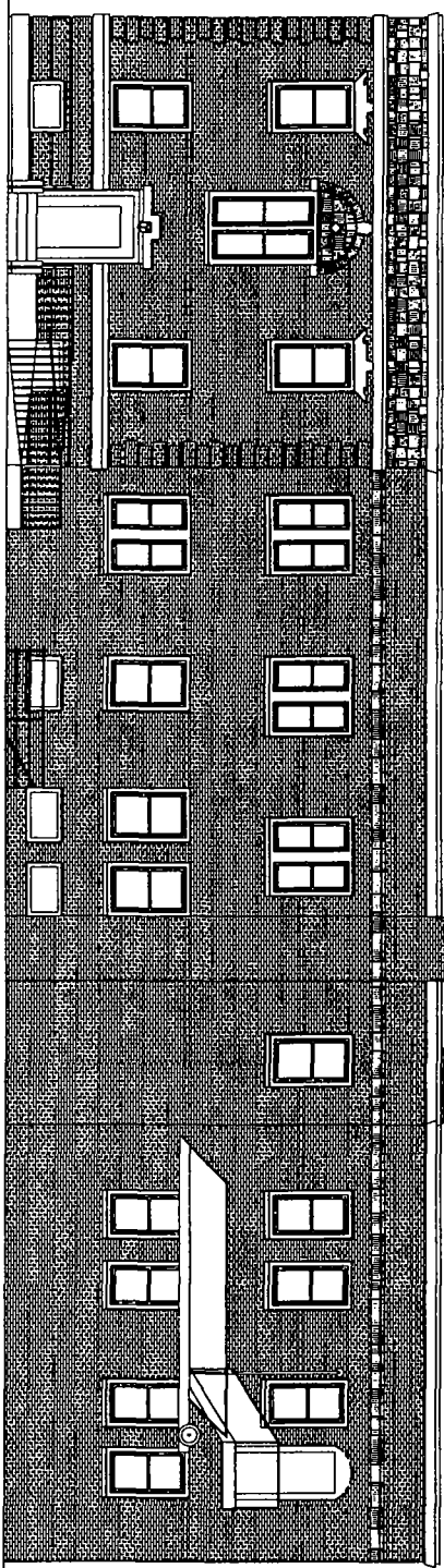
EAST ELEVATION SCALE: 3/32" = 1'-0"
