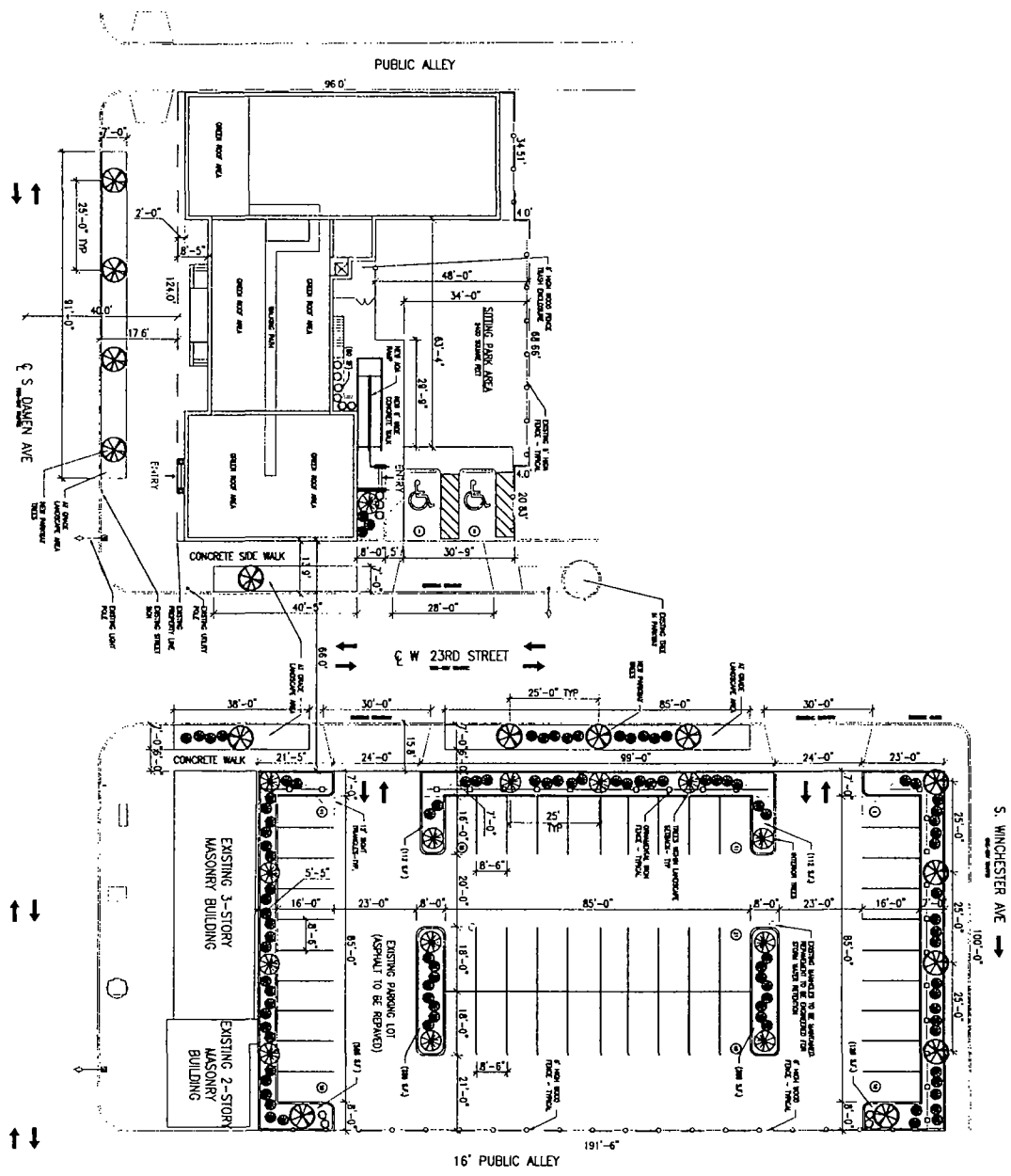
PROPOSED SITE PLAN SCALE: 1/32" = 1'-0"
