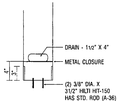
DETAIL - 4x6 TUBE 1 1/2" = 1'-0"
