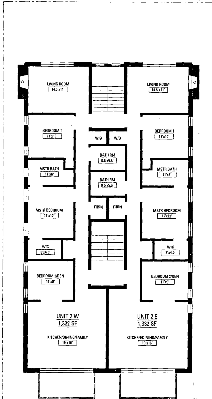
TYP. SECOND & THIRD FLOOR PLAN
