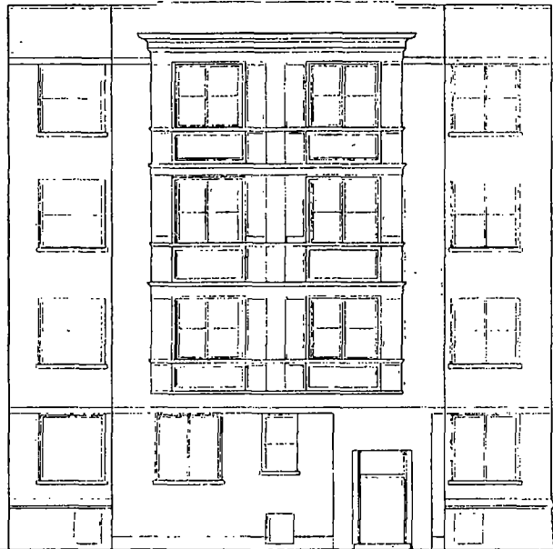
WEST ELEVATION (LA SALLE DR), 1/8" = 1'-0"
