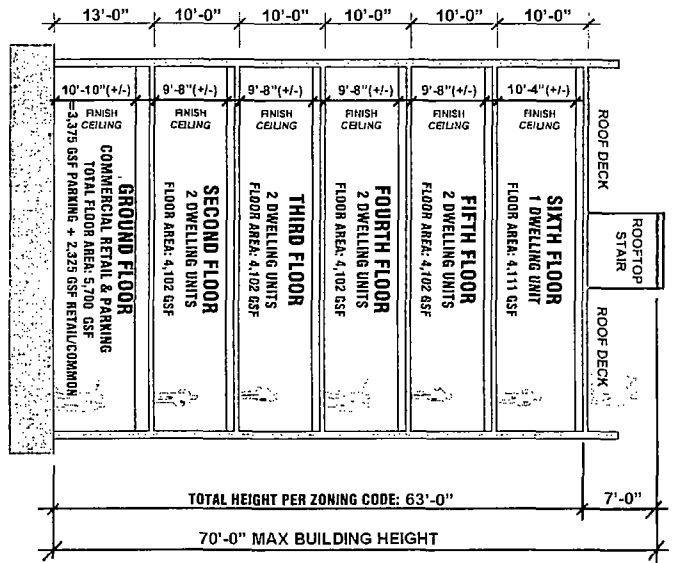
BUILDING SECTION
