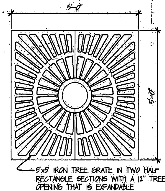
Detail Deciduous Tree Planting with Tree Grate in Concrete walk not to scale SIMILAR DETAIL IN RAISED SIDEWALK PLANTER.
