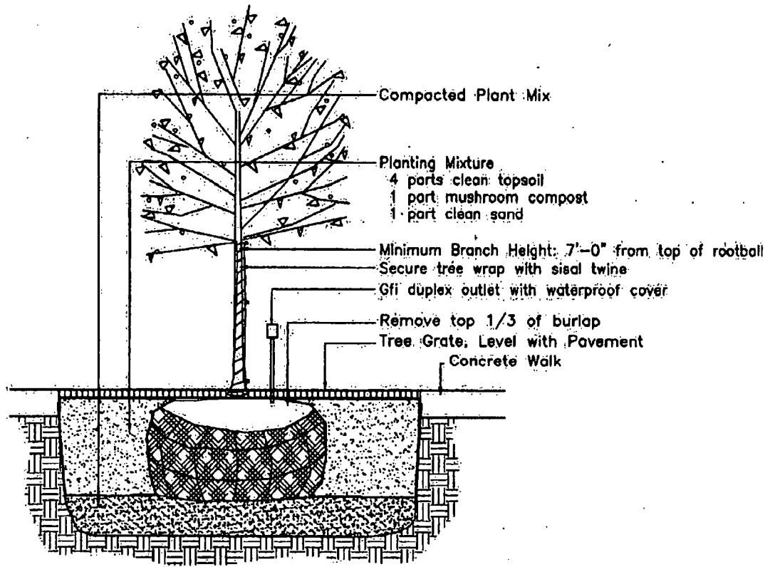
Detail Deciduous Tree Planting with Tree Grate in Concrete walk not to scale SIMILAR DETAIL IN RAISED SIDEWALK PLANTER.
