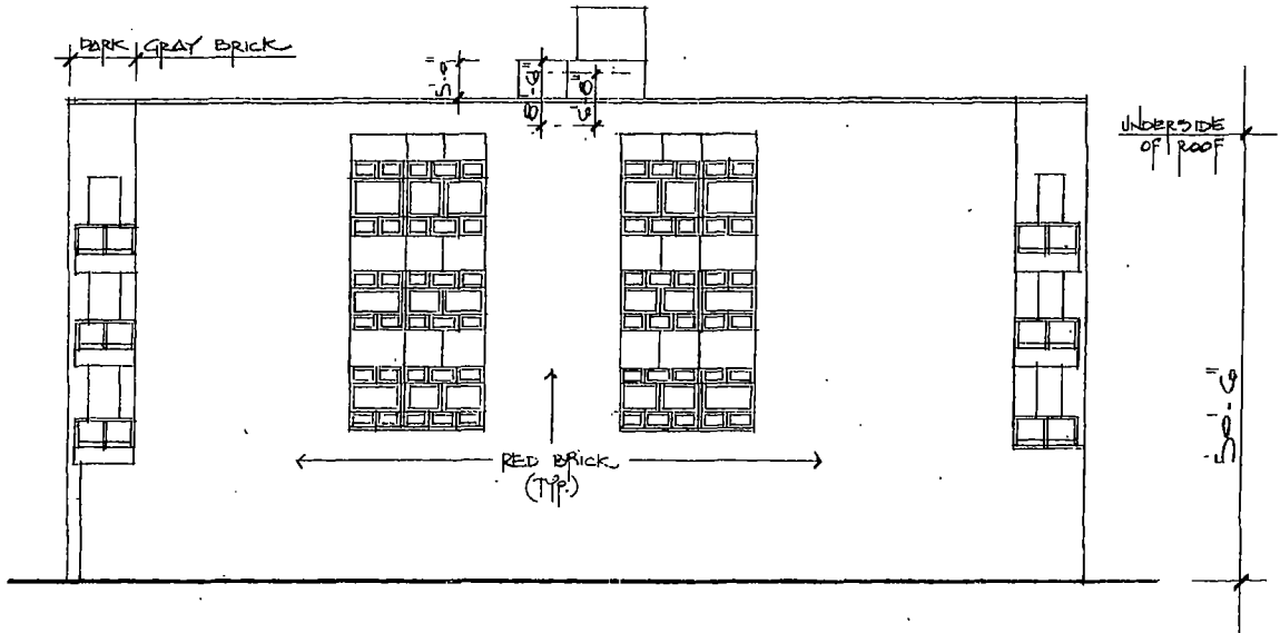
SOUTH ELEVATION 1/16" = 1'-0"
