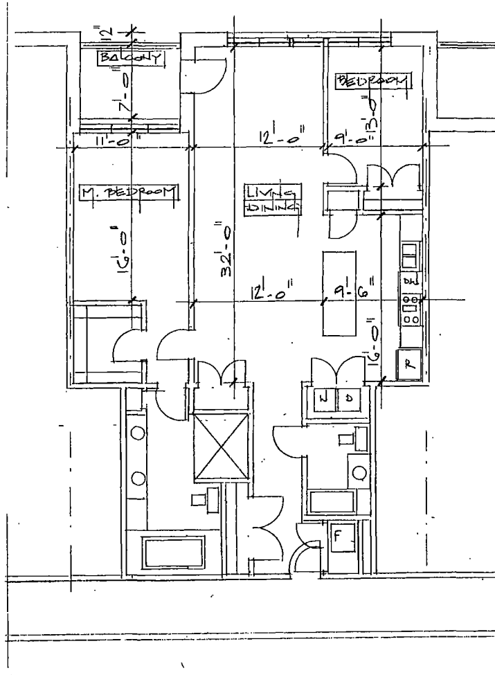
○ TYPICAL UNIT FLOOR PLAN 1350 S.F. WEST UNIT 1/8" = 1'-0"
