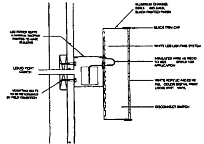
RACEWAY MOUNT INTERNALLY ILLUM CHANNEL LTR.
