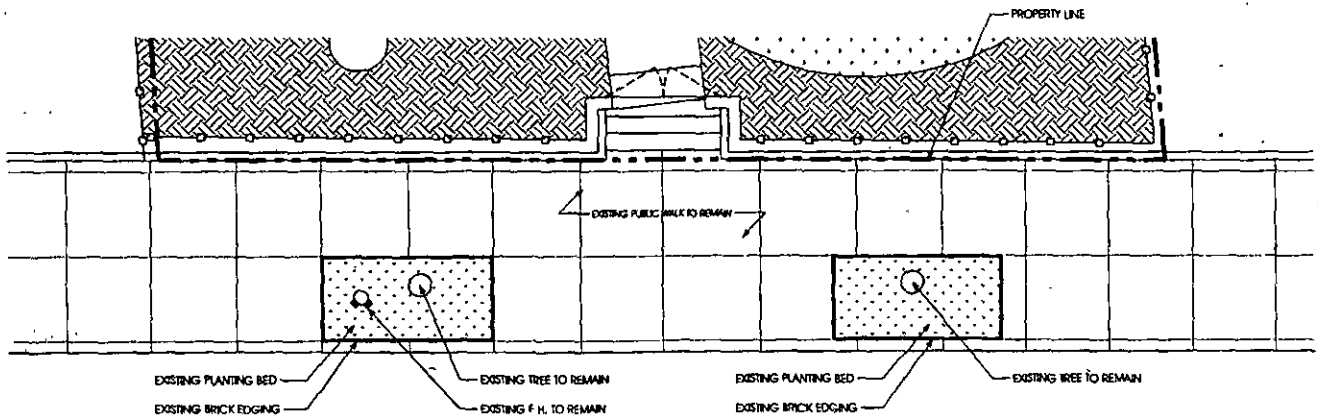
Existing Conditions - Public Way Sidewalk @ 526 West Deming
