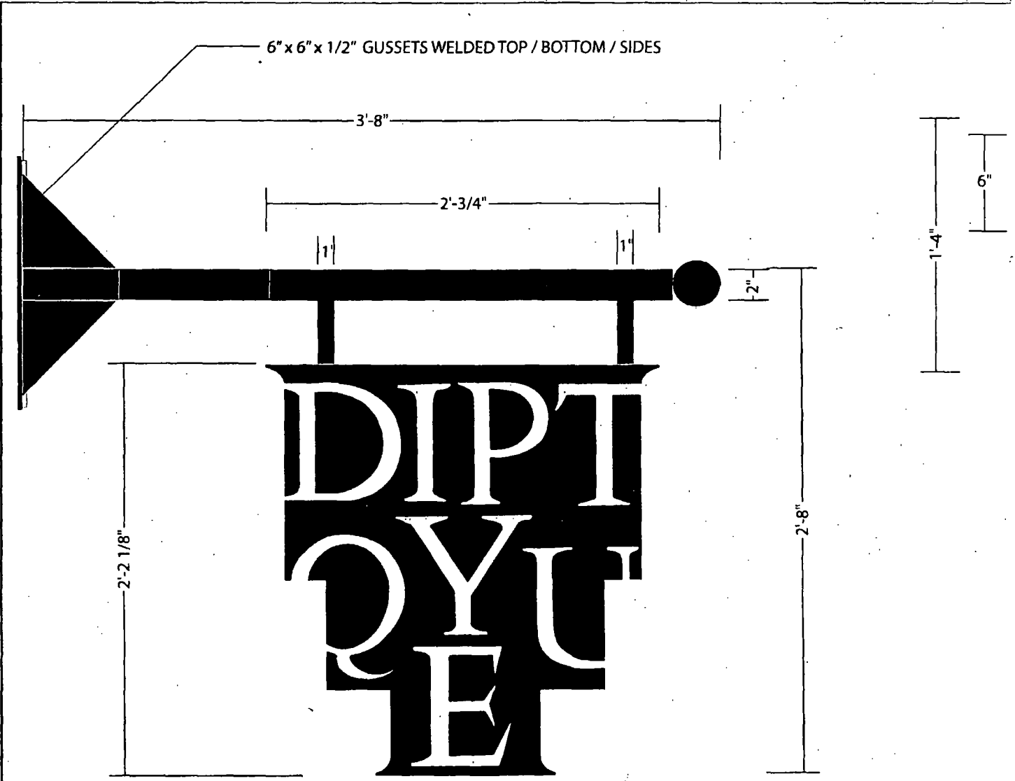
Front View 1 1/2 " = 1'-0"
