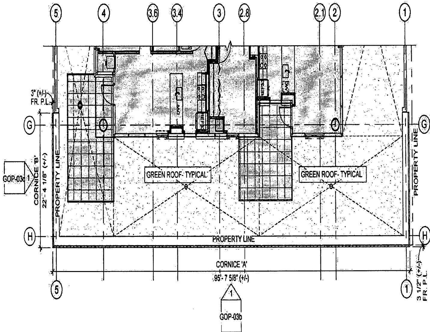
1 ENLARGED PLAN - PODIUM CORNICE PLAN \frac{3}{32}'' = 1'-0''
