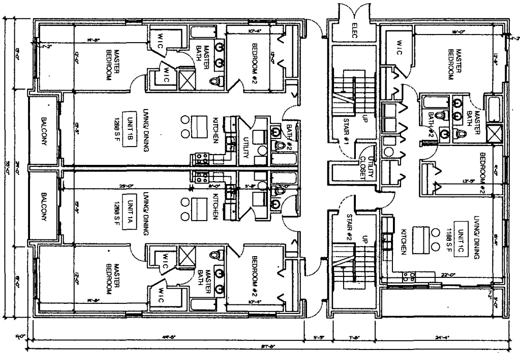
Second Floor Plan SCALE: 1/8" = 1'-0" Third floor similar
