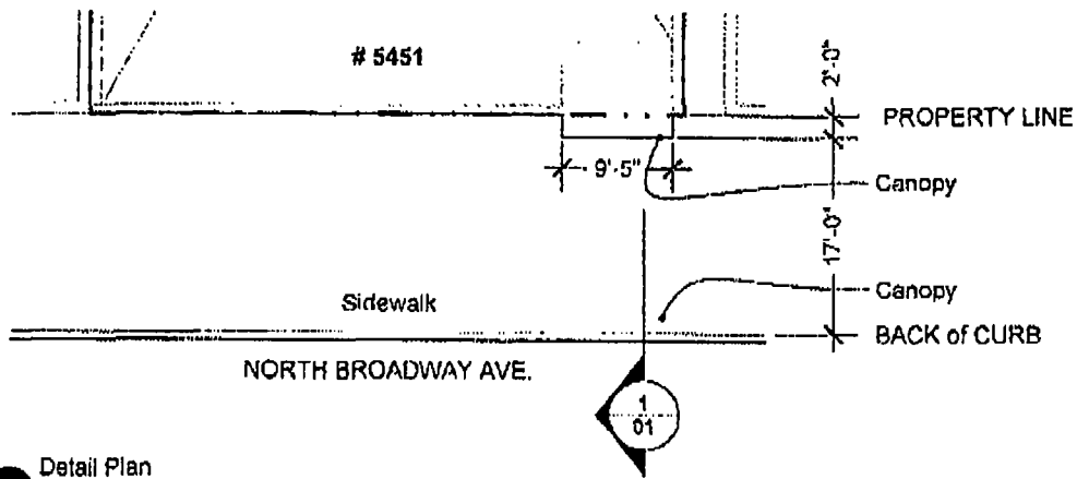
Detail Plan Scale: 1/10" = 1'
