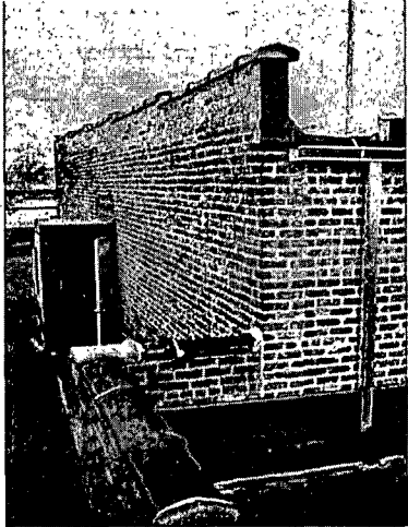
Fig. 25 – Dividing wall between lots 6, 7&8 and the rest of the building on roof, looking toward S. South Chicago Ave.
