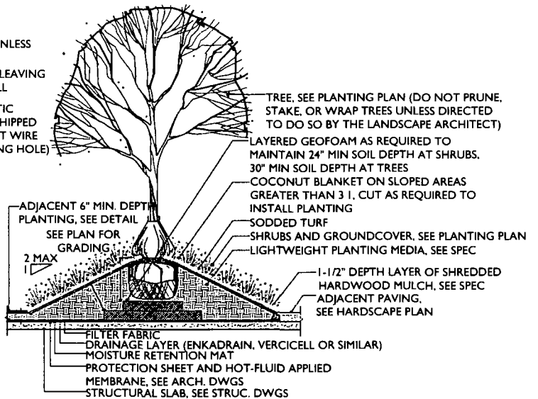
5 RAISED TREE PLANTING ON STRUCTURE N.T.S.
