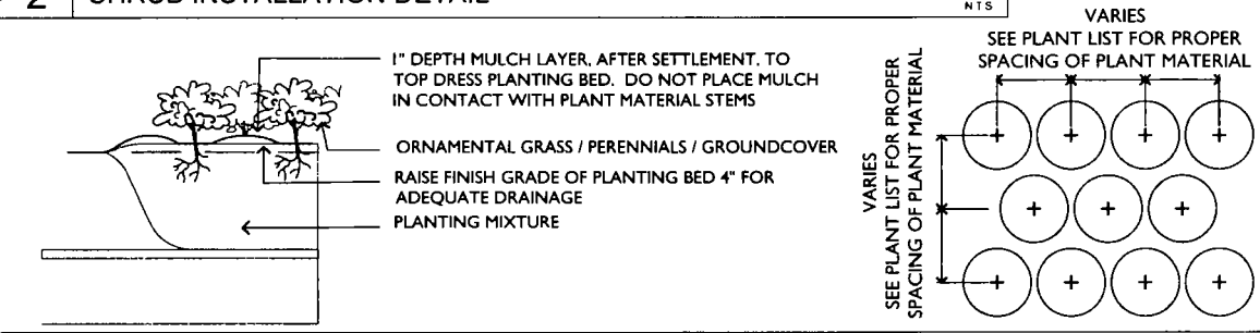
3 PERENNIALS INSTALLATION N.T.S.
