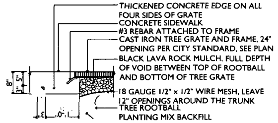
2 TREE GRATE ENLARGEMENT N.T.S.
