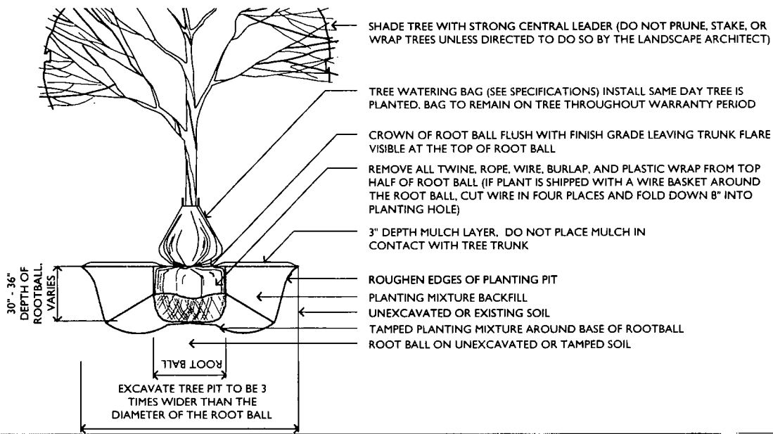
1 NEW TREE IN MULCH PLANTER DETAIL N.T.S.
