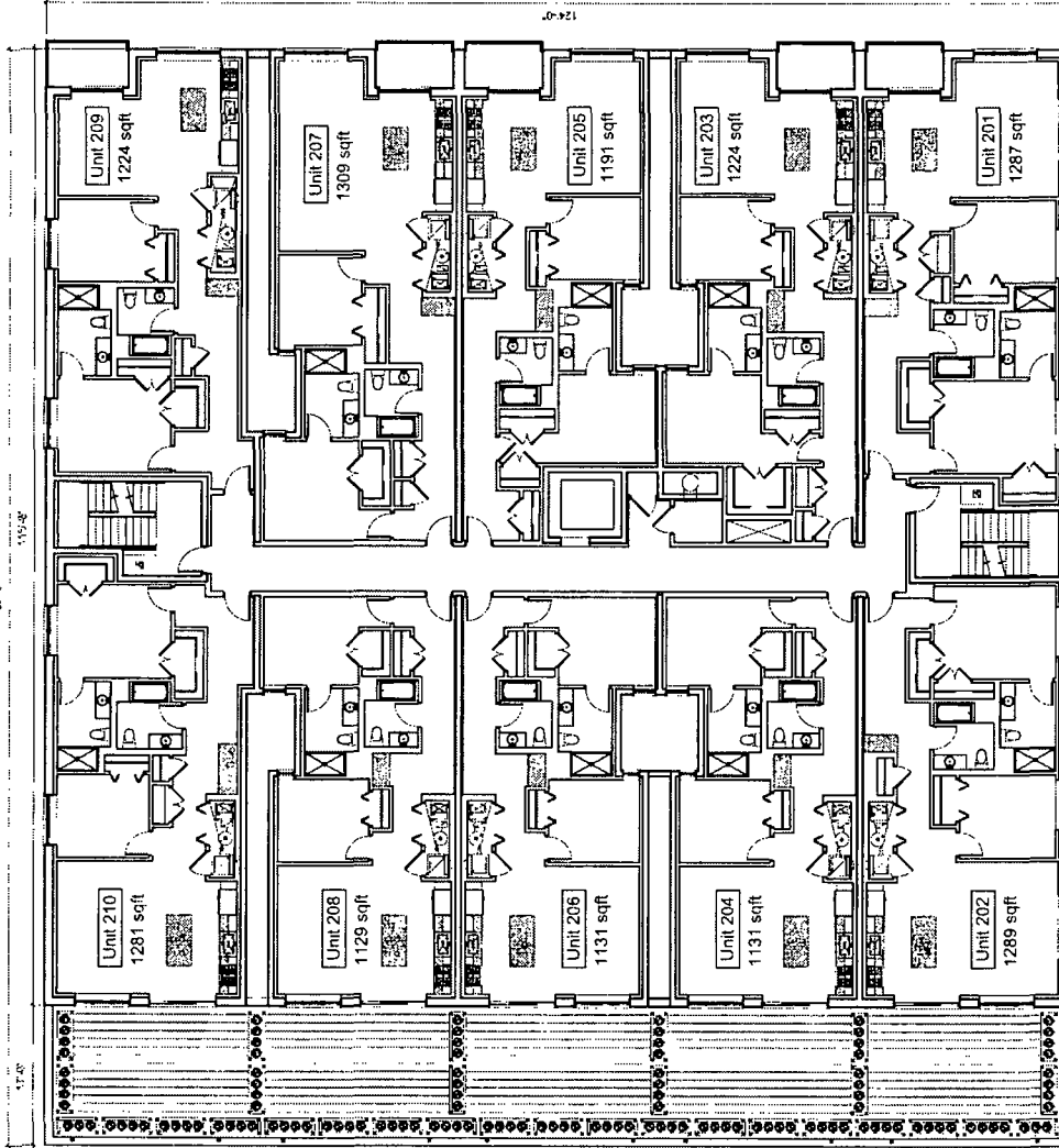
1 2nd Floor Plan N04 Scale: 1/8" = 1'-0"
