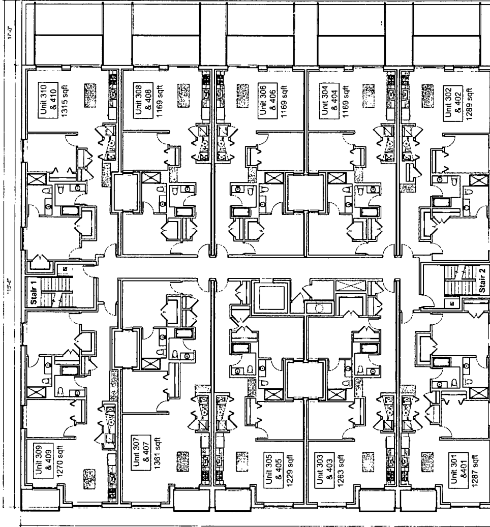
1 3rd & 4th Floor Plan Scale: 1/8" = 1'-0"
