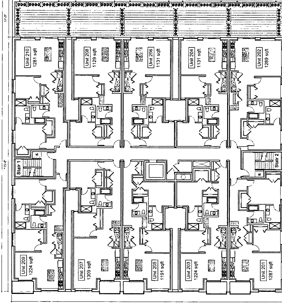
1 2nd Floor Plan Scale: 1/8" = 1'-0" MD4
