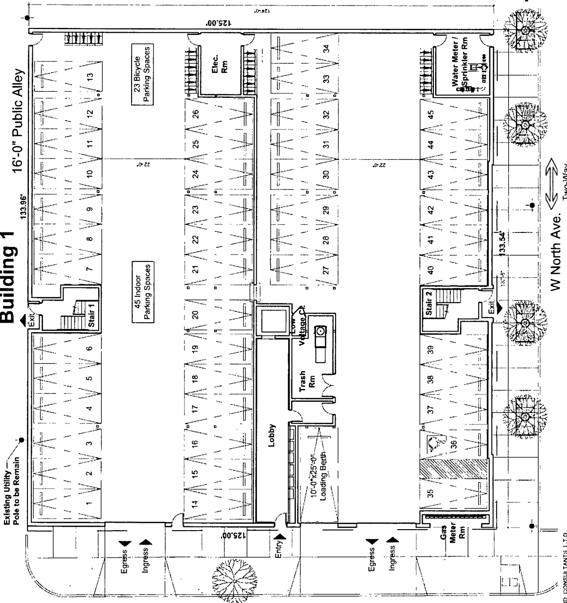
1 1st Floor Plan Scale: 1/8" = 1'-0"
