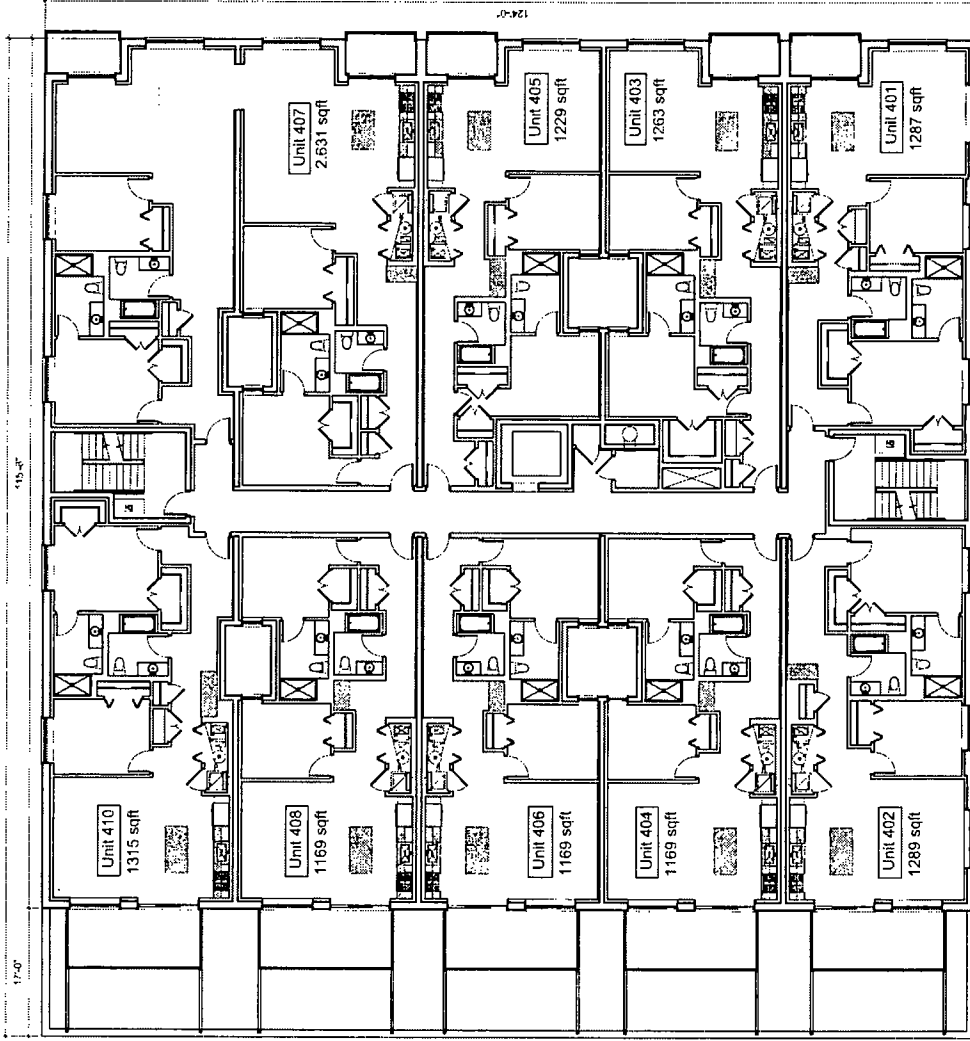
1 4th Floor Plan Scale: 1/4" = 1'-0"
