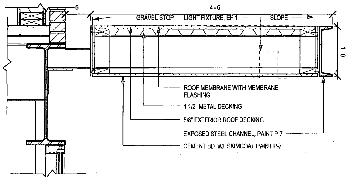
CANOPY DETAIL SCALE 1" = 1'-0"
