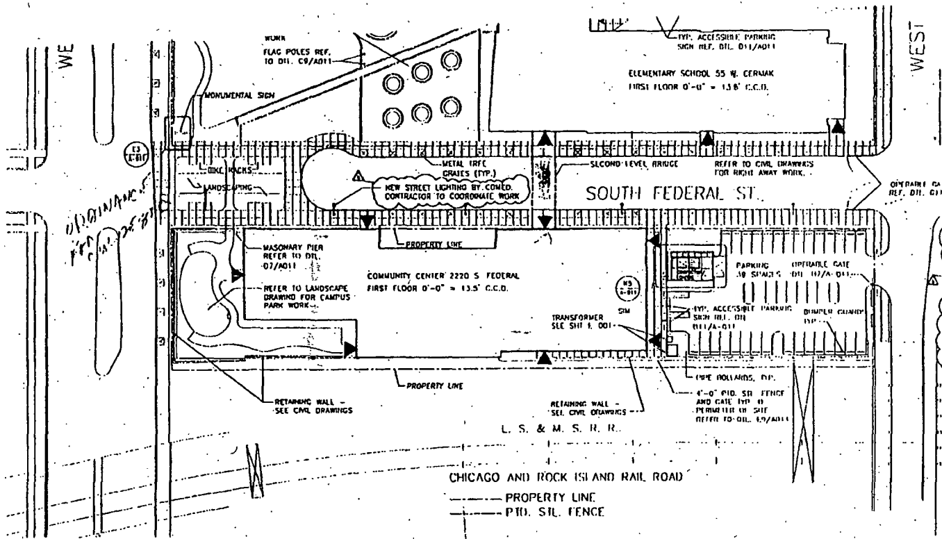
K10 SITE PLAN SCALE 1/8" = 1'-0"
