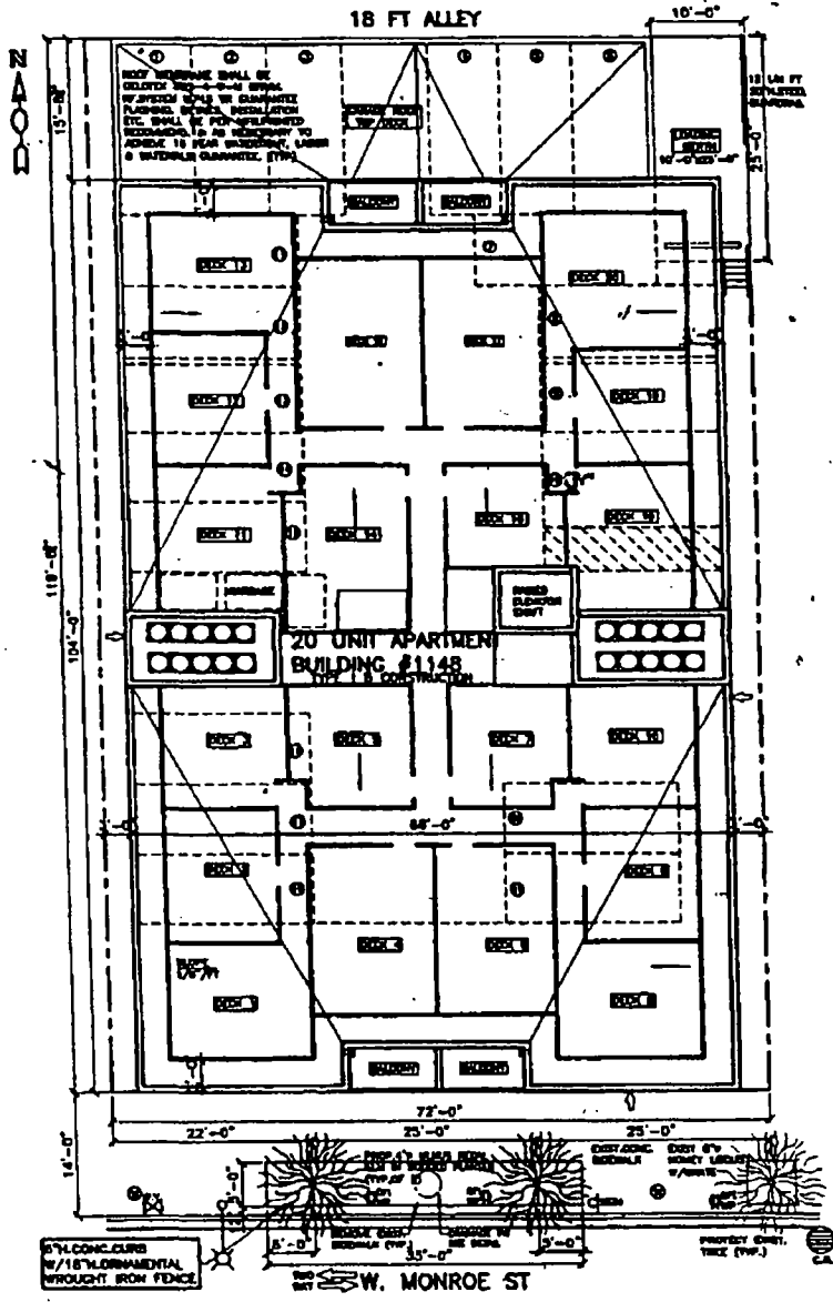
⊕ SITE/ROOF PLAN SCALE: 1" = 10'-0"
