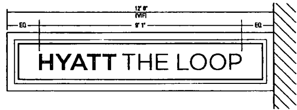
Canopy Side Elevation (East) 1/2" = 1'-0"
