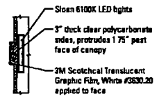
Section (Typical) 1/2" = 1'-0"
