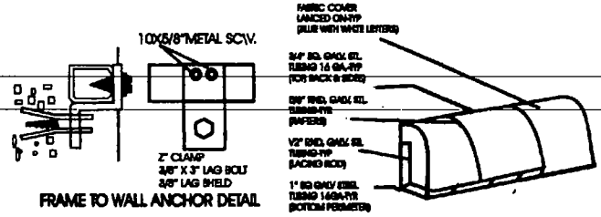
Side & elevation details
