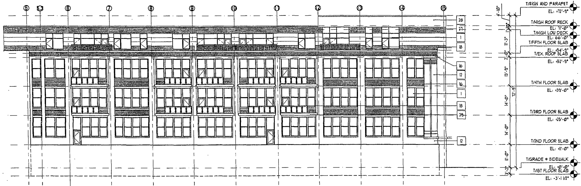
1 ELEVATION: EAST COURTYARD SCALE: NTS
