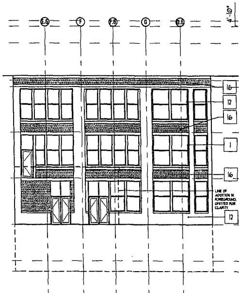
1 ELEVATION: NORTH COURTYARD SCALE: NTS
