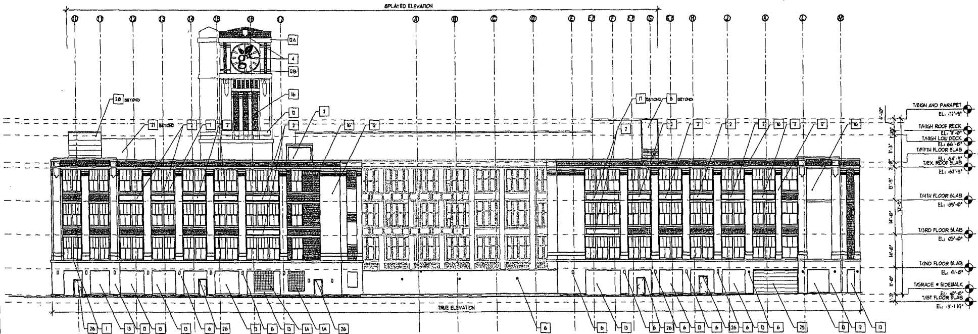
1 ELEVATION: SOUTHWEST (EXPRESSWAY) SCALE: NTS
