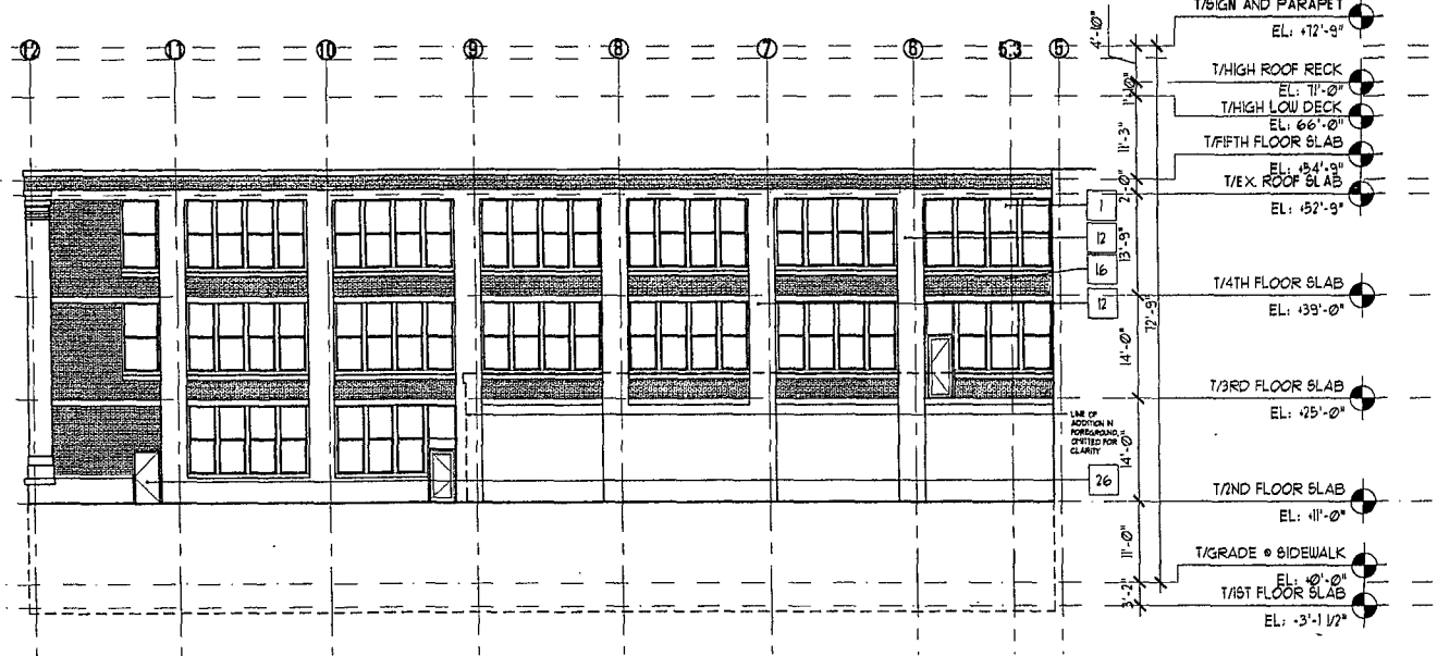
2 ELEVATION: WEST COURTYARD SCALE: NTS
