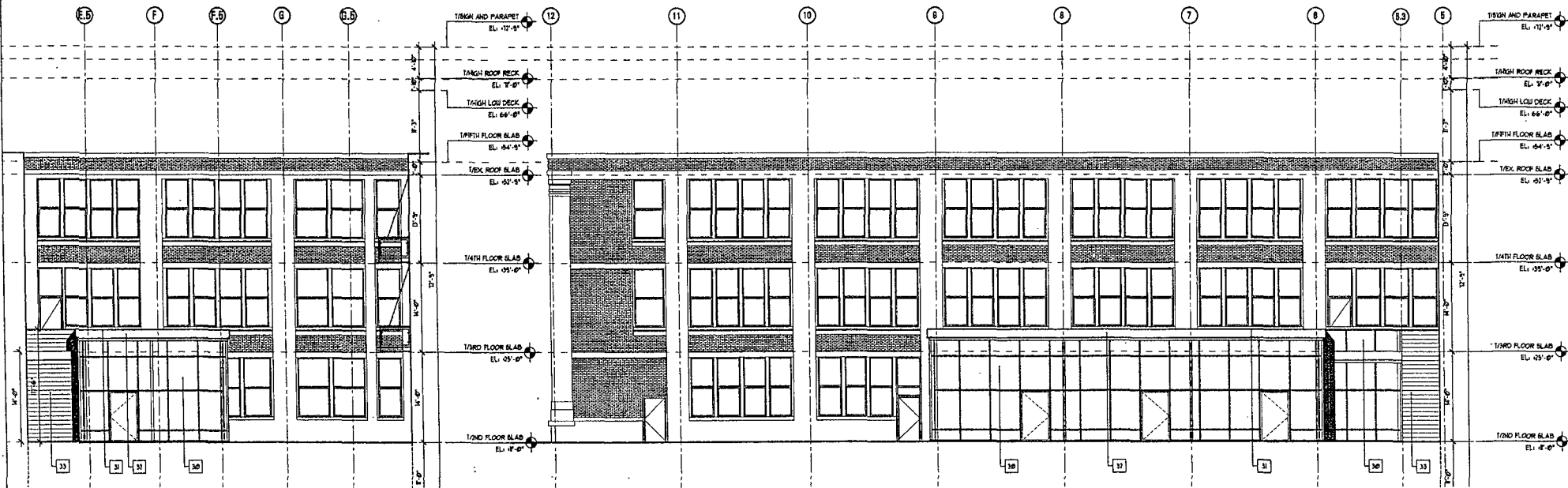
1 ELEVATION: SOUTH COURTYARD ADDITION SCALE: NTS
