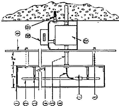
REVERSE-ILLUMINATED CHANNEL LETTERS W/ BACKPANEL, RACEWAY-MOUNTED
